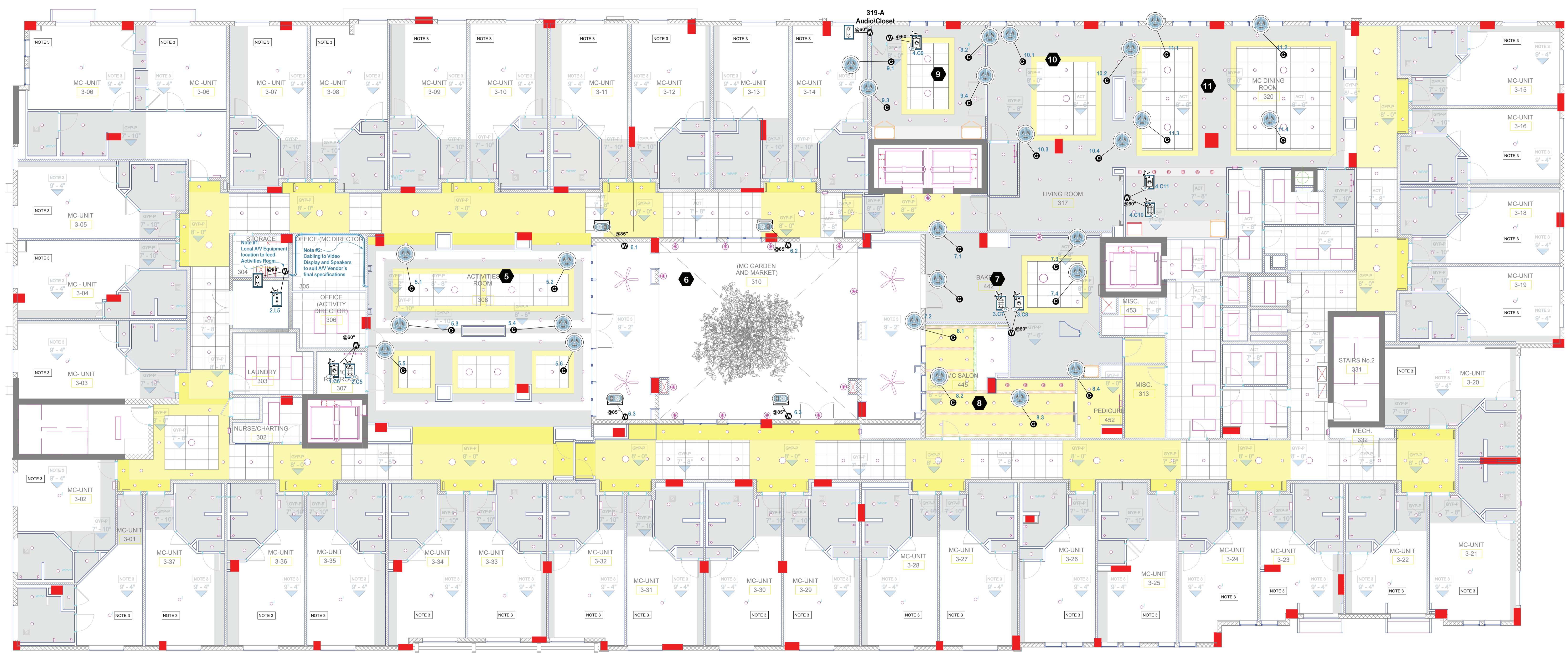
1 3RD FLOOR OVERALL REFLECTED CEILING PLAN A-4-300 / 1/8" = 1'-0"
